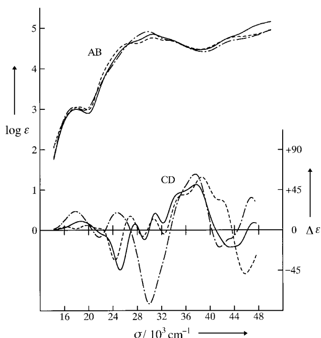
Figure 2. Electronic absorption (AB) and CD spectra of (+)\text{^{260}}-(A)_2\text{-[1]}^{2+} \times 2 (•—•), (+)\text{^{260}}-(A)_4\text{-[2]}^{6+} (---), and (+)\text{^{260}}-(A)_4\text{-[3]}^{6+} (—) in \text{H}_2\text{O} .
